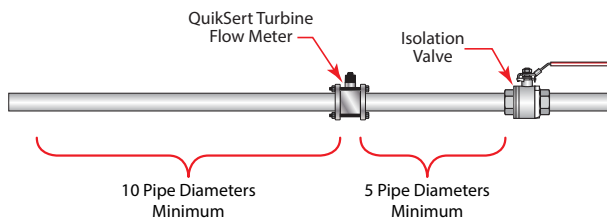
Figure 3: Meter installation without using a bypass line
