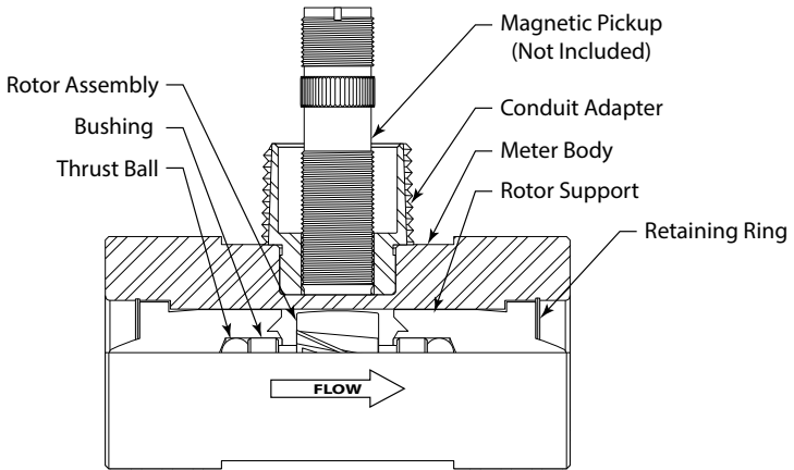
Figure 4: Typical cross-section of models B131C-038 through B131-100
