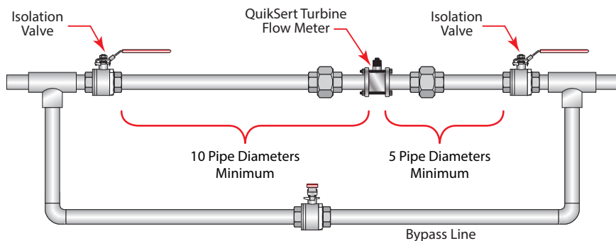
Figure 2: Meter installation using a bypass line
