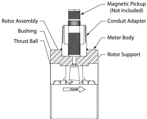
Figure 5: Typical cross-section of models B132C-050...B139C-900
