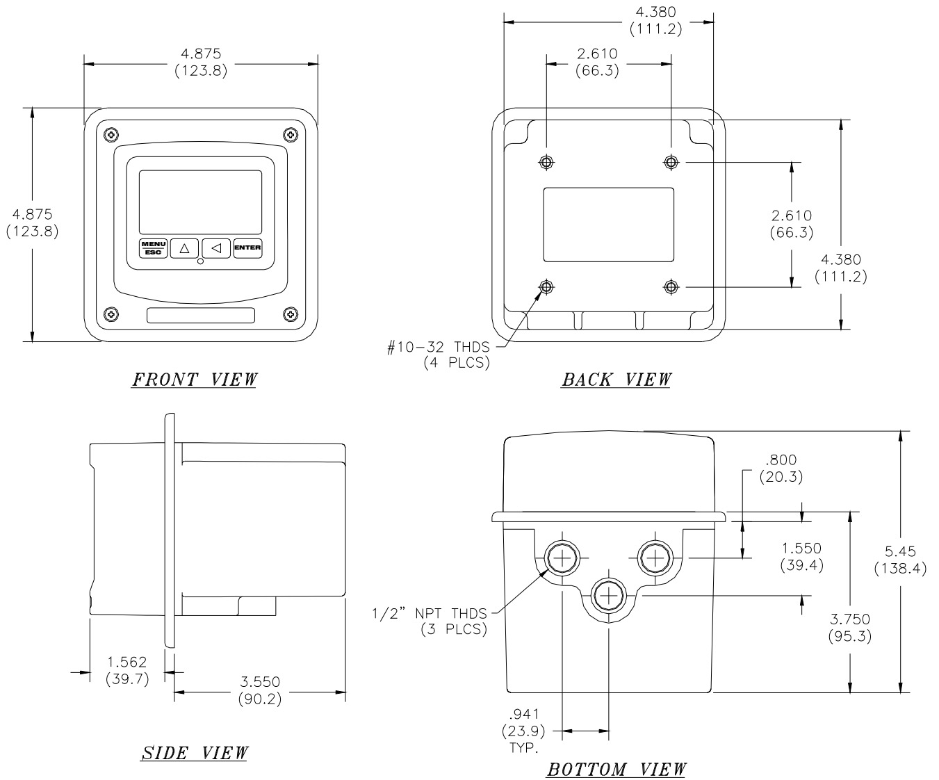
Figure 1 - Q45 Enclosure Dimensions, AC Powered Units
