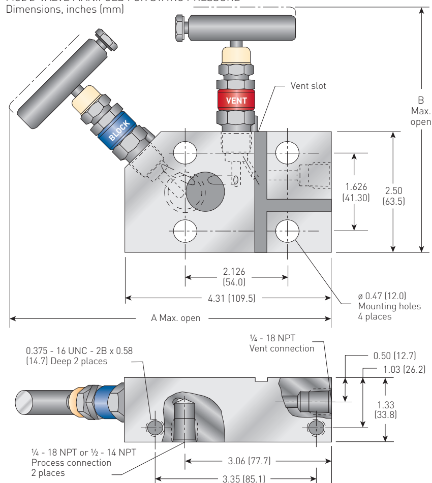
MC2 2-VALVE MANIFOLD FOR STATIC PRESSURE Dimensions, inches (mm)
