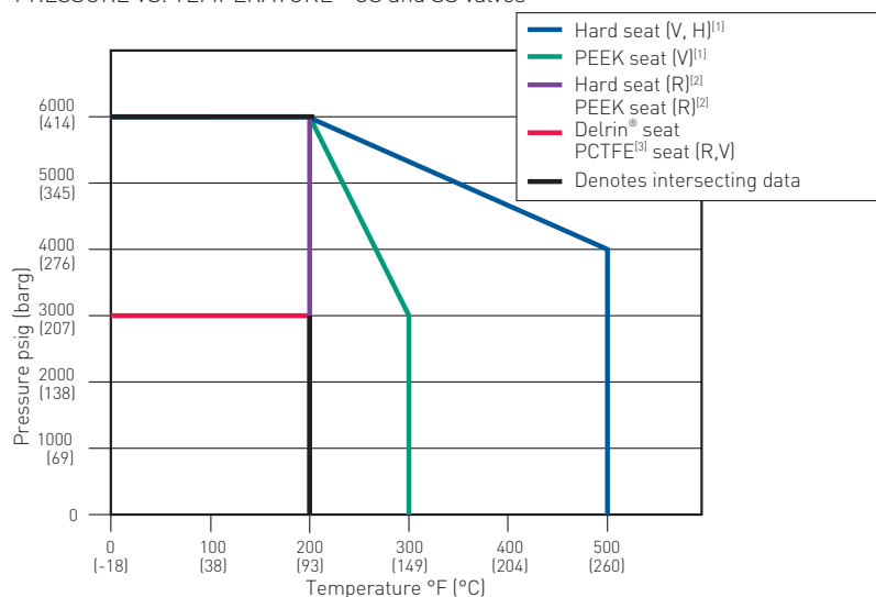
PRESSURE VS. TEMPERATURE - CS and SS valves
