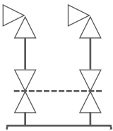
Interlocking block valve with two vessel penetrations
