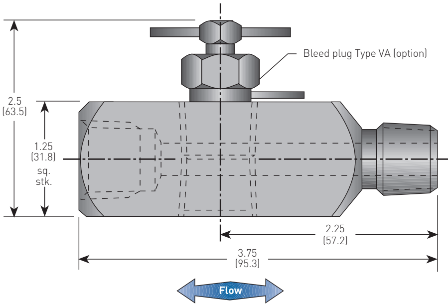
BLEED TEE DIMENSIONS, inches (mm)
