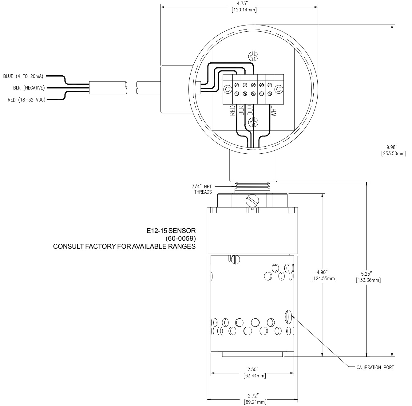
SENSOR WITH OPTIONAL JUNCTION BOX (00-1752)
